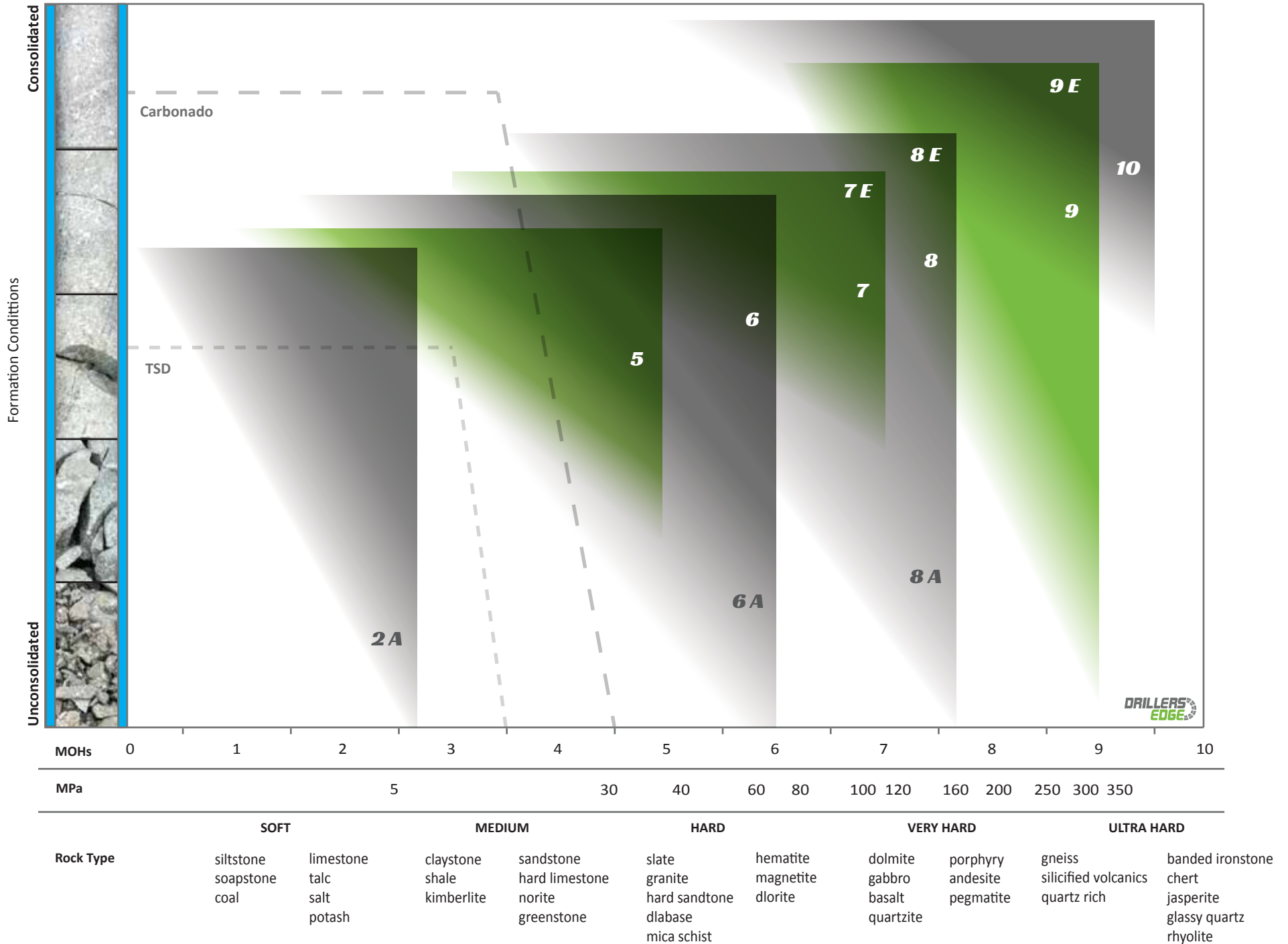
Mineral Exploration Bit Selection Chart
